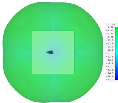
UHF-element 380 MHz
