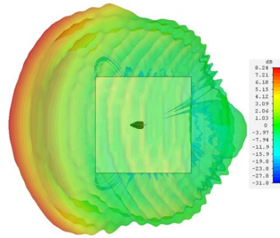
WIFI-element 5600 MHz
