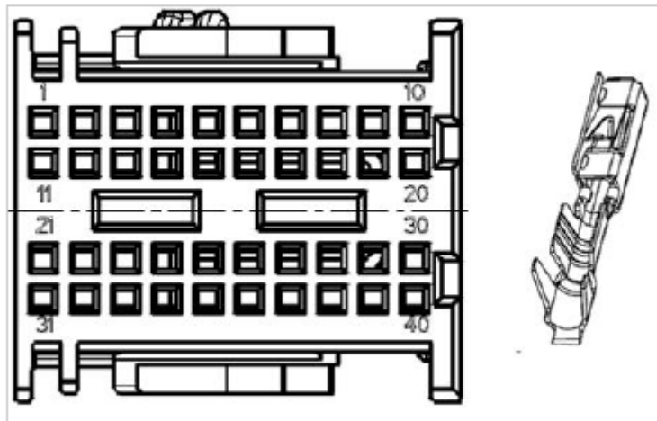
Plug and contact socket
